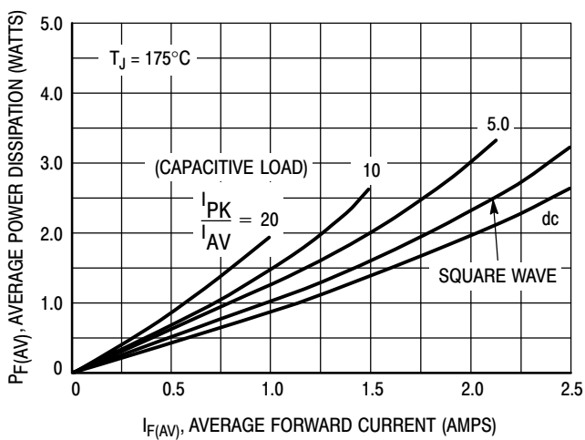
Figure 9. Power Dissipation
