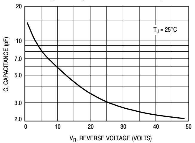
Figure 10. Typical Capacitance
