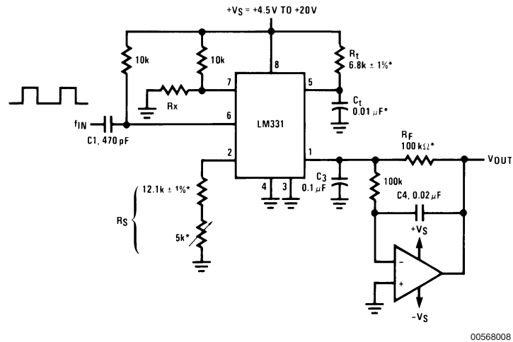
FIGURE 6. Simple Frequency-to-Voltage Converter, 10 kHz Full-Scale, ±0.06% Non-Linearity
