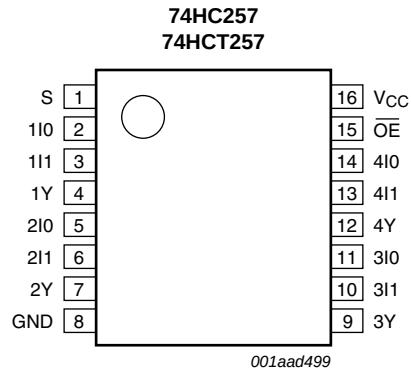
Fig 5. Pin configuration DIP16, SO16, SSOP16 and TSSOP16
