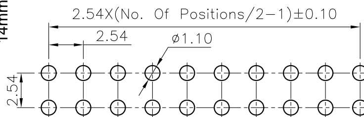
PCB Layout
