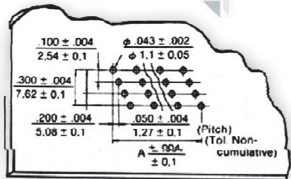
Aligned P.C. Board Hole Detail
