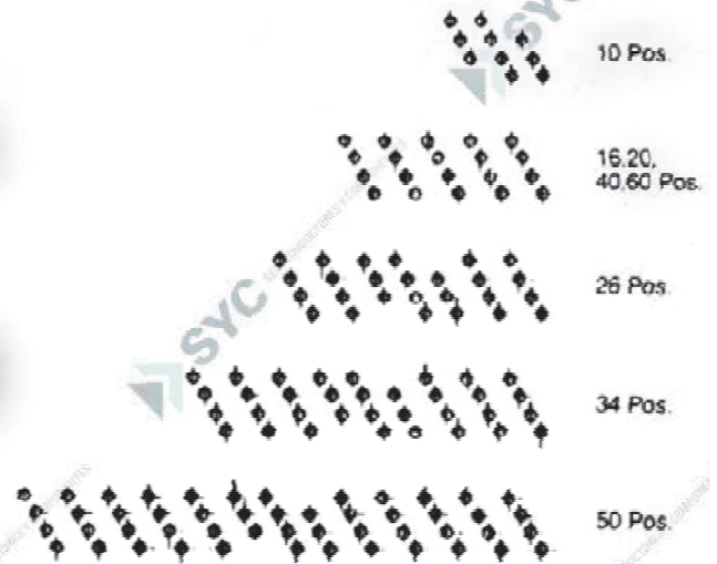
Aligned P.C. Board Hole Detail
