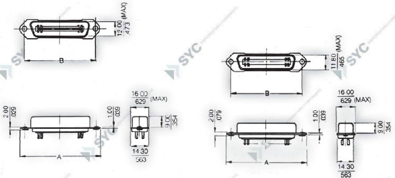
Plug
