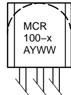
TO-92 (TO-226) CASE 029 STYLE 10
