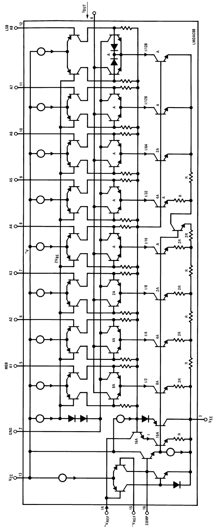
FIGURE 2. Equivalent Circuit of the DAC0808 Series (Note 8)
