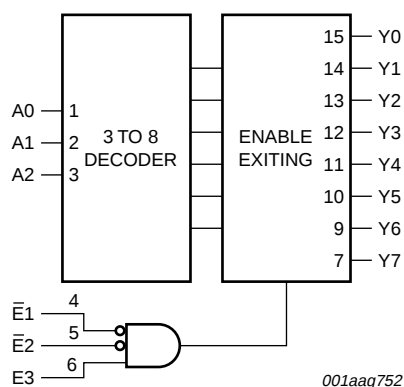
Fig 1. Logic symbol
