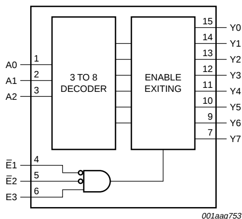
Fig 2. Functional diagram
