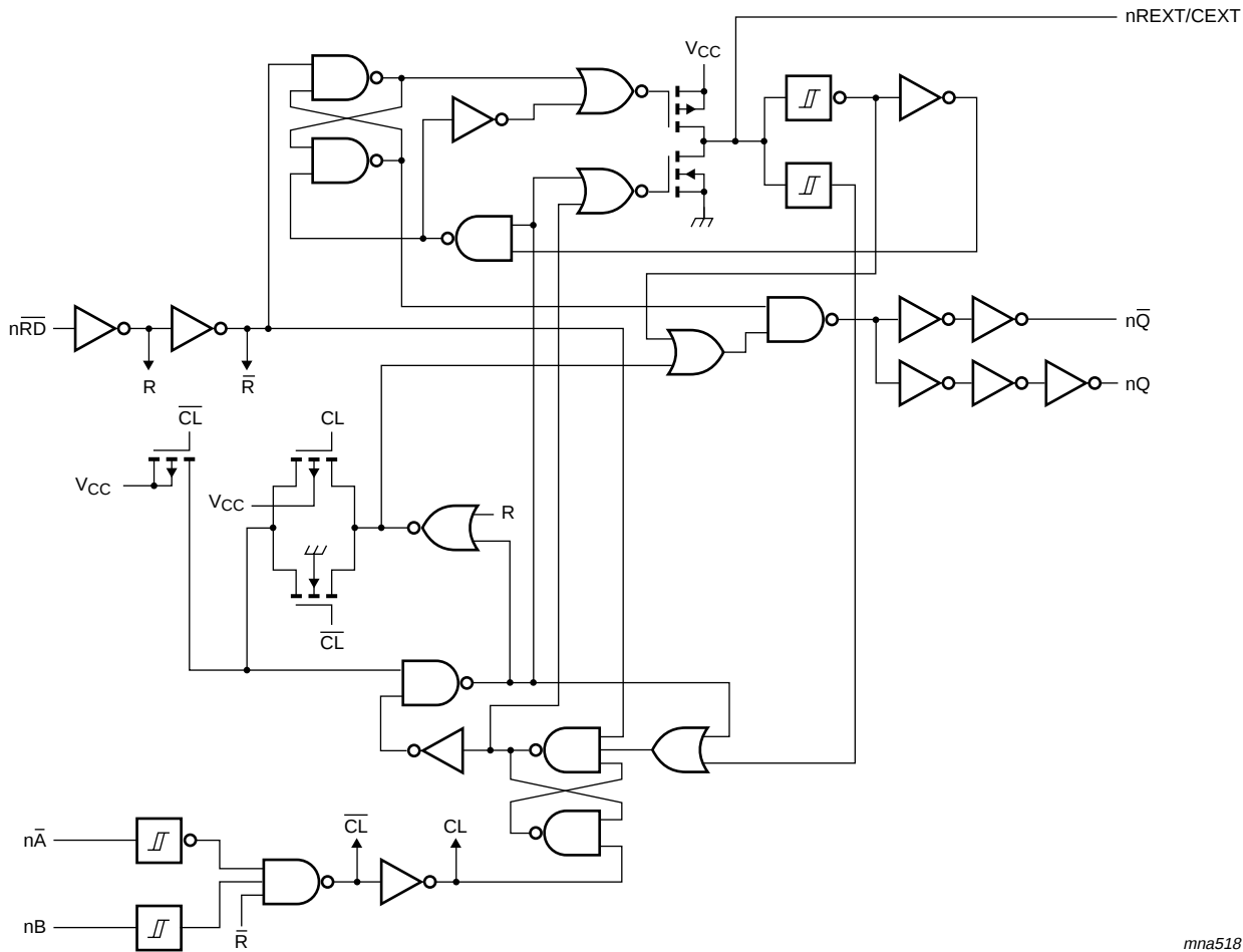
Fig 4. Logic diagram
