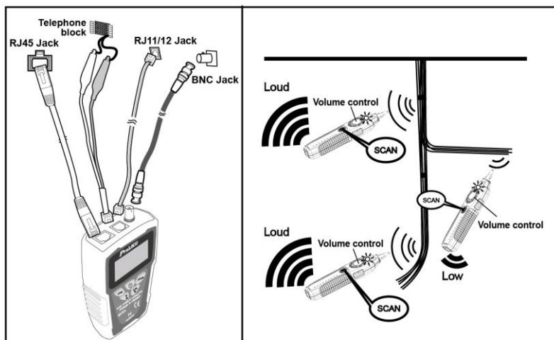
Figure 9 Isolating Cable
