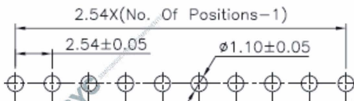
PCB Layout
