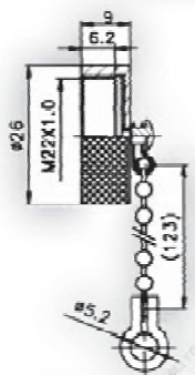
PLS-20-GPM3/8"
