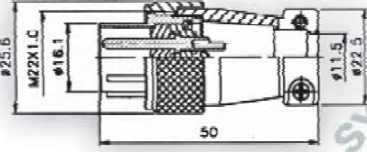
PLS-20-PM
