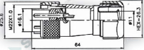
PLS-20-GPM3/8"
