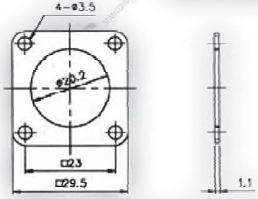
RUBBER PLATE FOR PLS-20-RF
