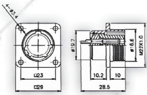
PLS-20-RF
