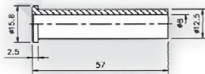
RUBBER TUBE FOR PLS-20-PF
