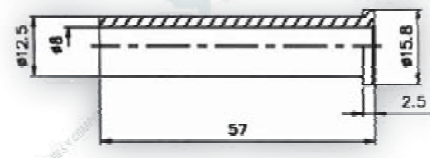
RUBBER TUBE FOR PLS-20-PM
