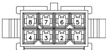
8PIN
