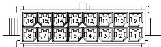
16PIN
