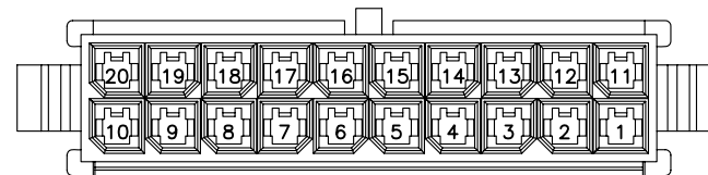
20PIN
